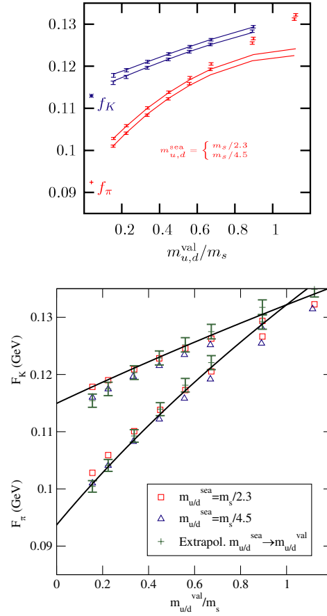
FIG. 1 (color online). (a) Lattice results for F_\pi and F_K and \chi PT extrapolations taken from MILC Collaboration. (b) Comparison of the Lattice results [7] with the R\chi T extrapolations for the values from the fit, F = 93.7 MeV, M_S = 1020 MeV and the splitting e_m^S = -0.02 . The kaon mass varies as m_K^2 = (m_K^{\text{Phys}})^2 + [m_\pi^2 - (m_\pi^{\text{Phys}})^2]/2 due to its light-quark content. They are shown together with the data for m_{u,d}^{\text{sea}} = m_s/2.3 (squares), m_{u,d}^{\text{sea}} = m_s/4.5 (triangles) and the linear extrapolation to the value m_{u,d}^{\text{sea}} = m_{u,d}^{\text{val}} (error bars).
